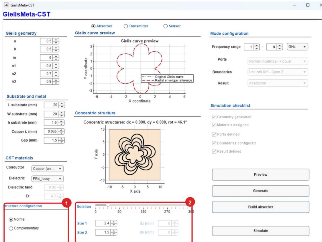
Figure 7. Absorber size and rotation settings.
