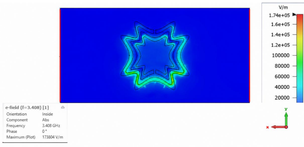
Figure 20. Electric-field distribution of the sensor structure at 3.408 GHz. Lighter colors indicate higher field magnitude; the scale on the right is given in V/m.
