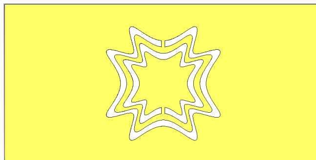
Figure 18. CST Studio Suite view of the generated complementary sensor model.
