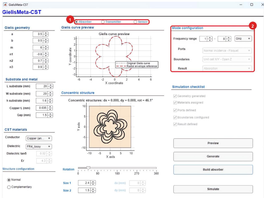
Figure 2. Absorber-mode selection and automatically assigned configuration.
