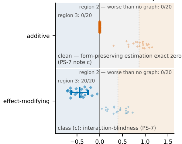
collider · linear · four-way
