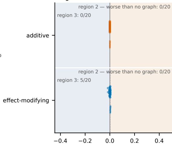
chain · nonlinear-Gaussian · four-way
