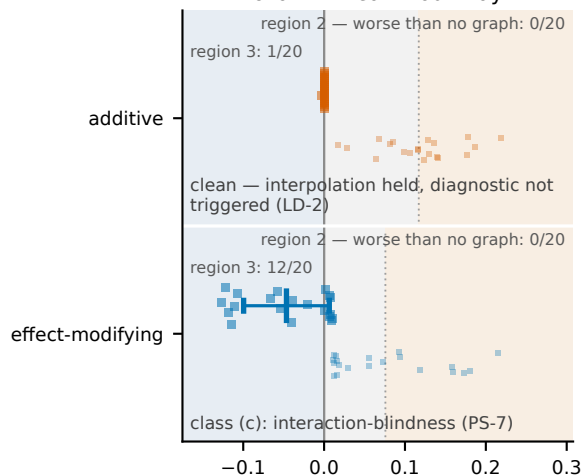
collider · linear · four-way
