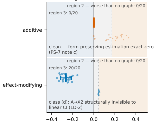
chain · linear · four-way
