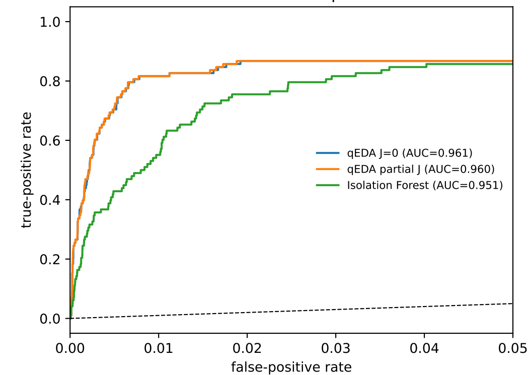
ROC detail at low false-positive rates
