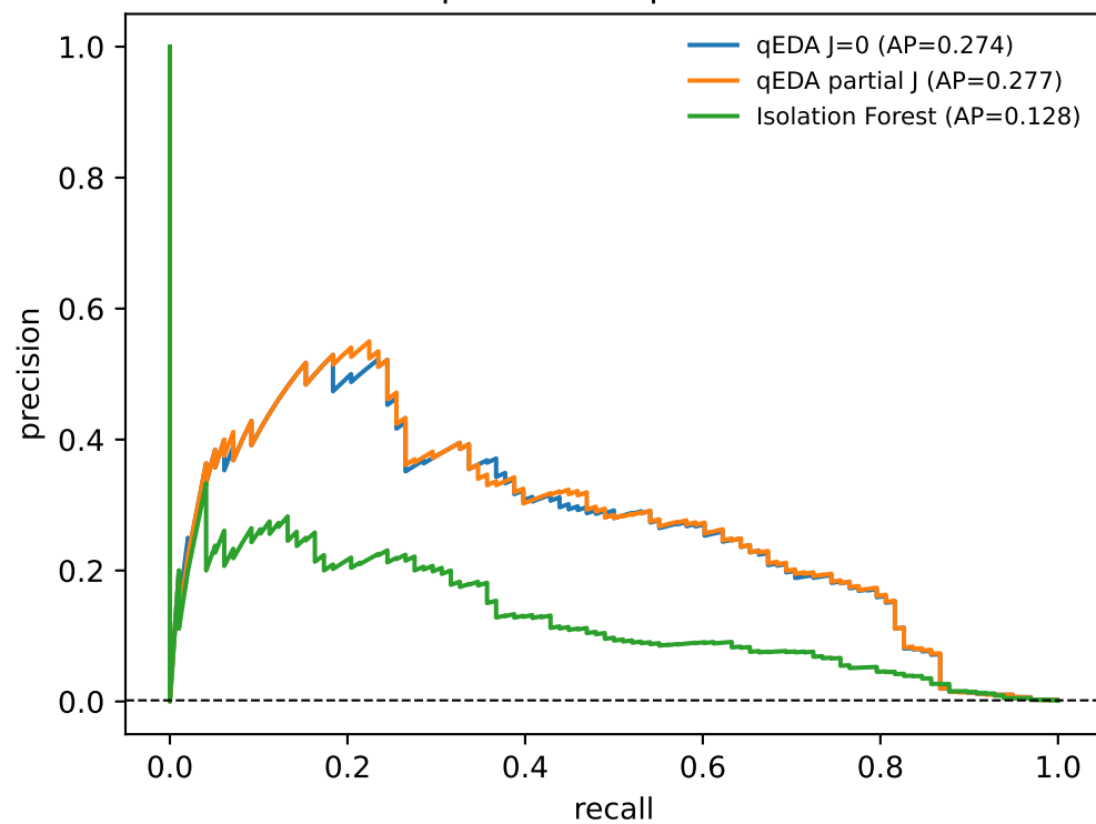
Variability across 120 balanced marginals
