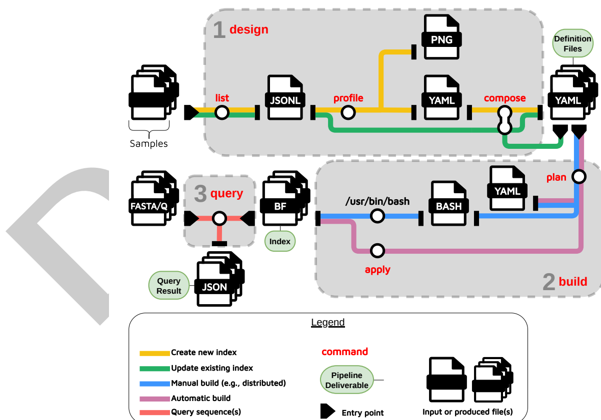
Figure 1: Overview of the kmhelpers workflow
