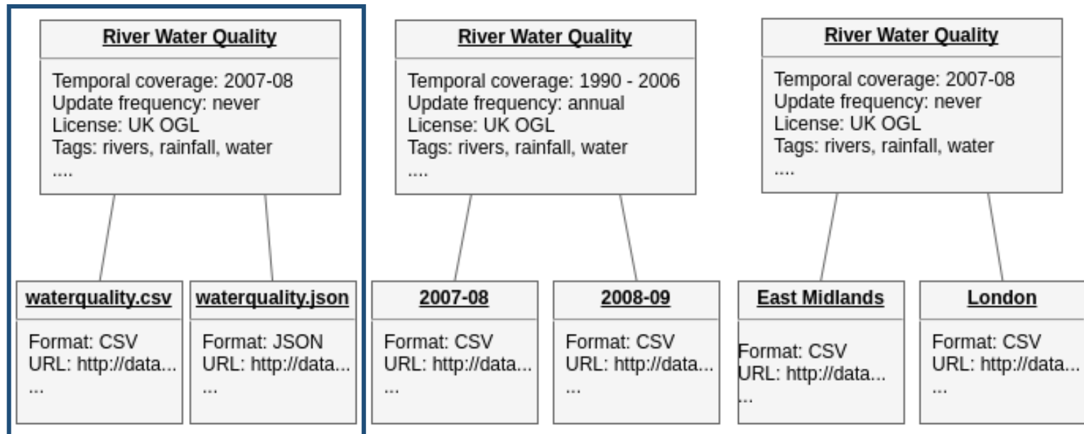
DCAT distribution
