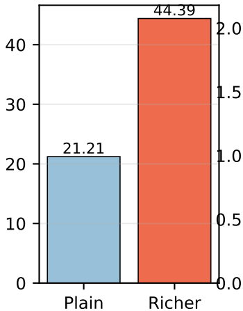
Sensitivity
