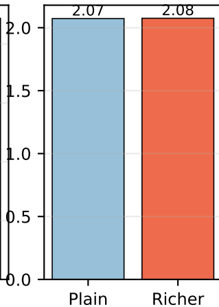
Entropy
