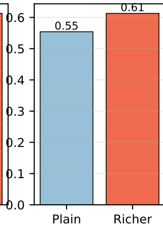
Rank stability
