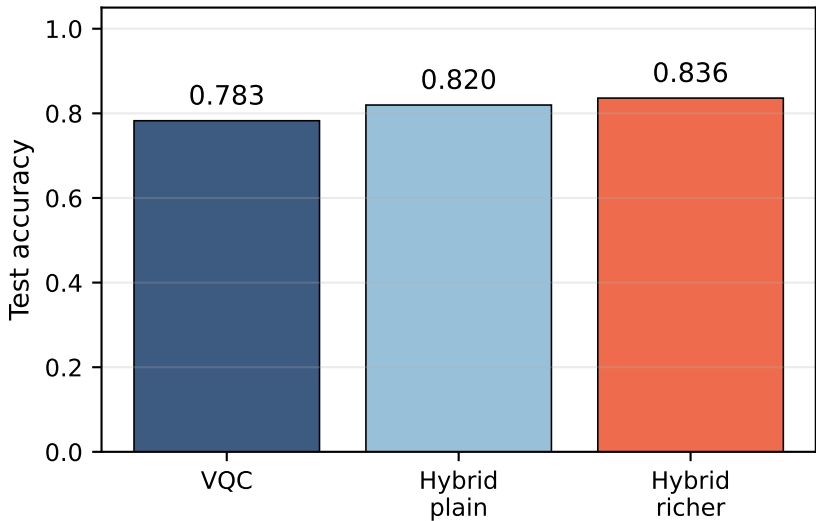
Cleveland Test Accuracy
