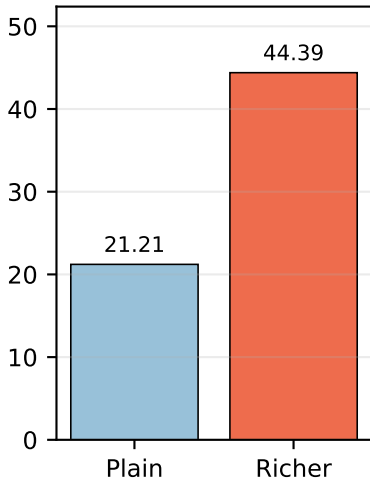
Sensitivity
