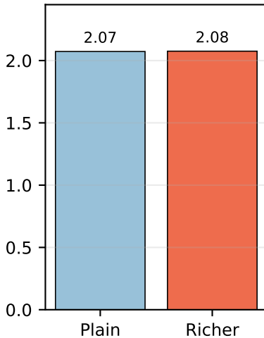
Entropy
