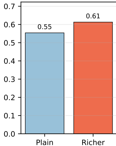
Rank stability
