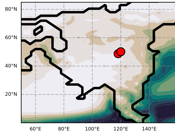
HadCM3+Getech 1120
