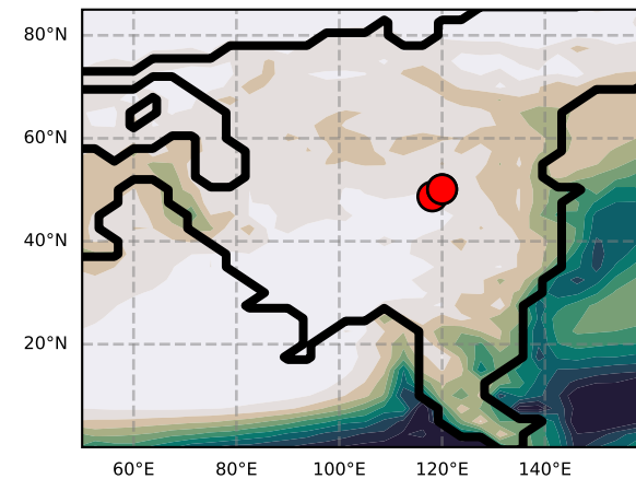
HadCM3+Getech 1120
