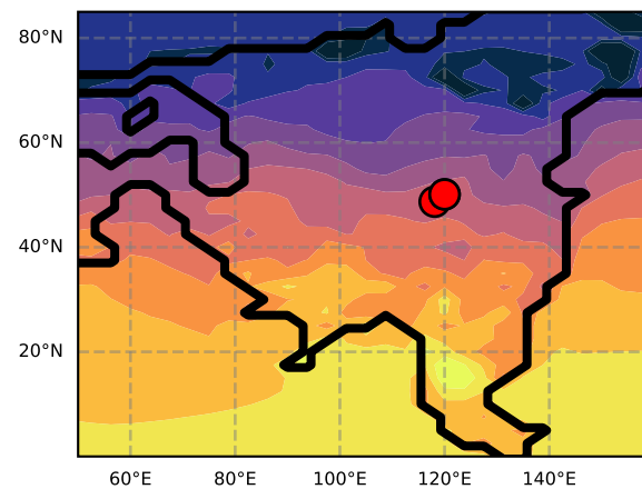
HadCM3+Getech 1120
