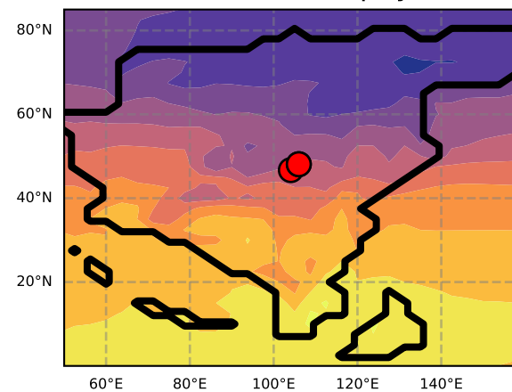
HadCM3+Scotese+phys 1103
