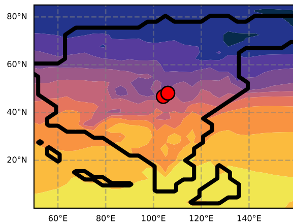
HadCM3+Scotese 1103
