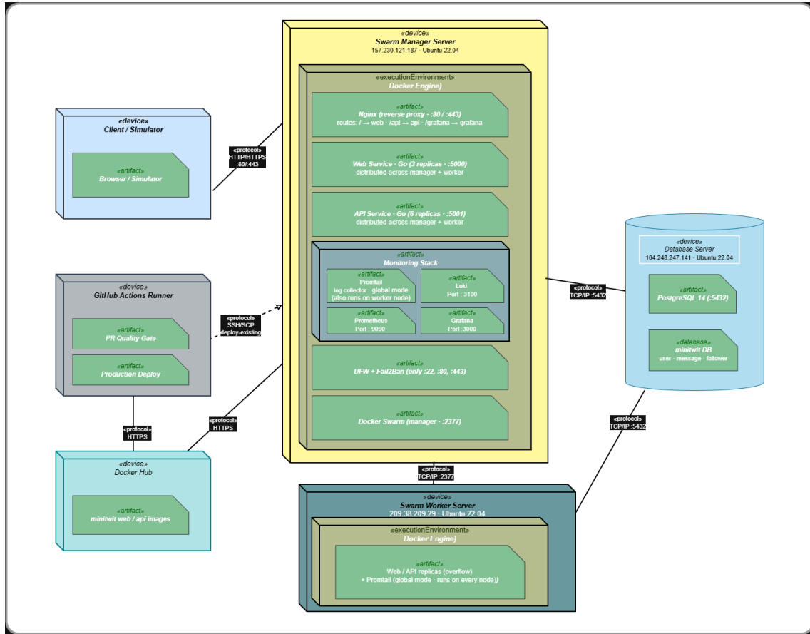
Figure 1: Deployment diagram of the MiniTwit system
