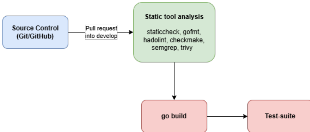
Figure 4: Overview of the PR Quality gate pipeline
