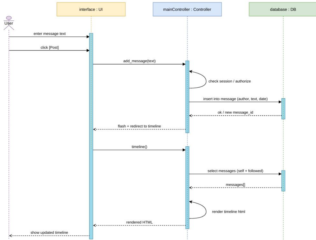
Figure 2: Post creation and timeline rendering sequence diagram
