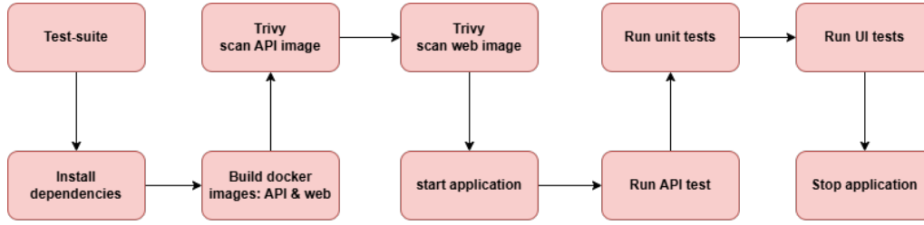
Figure 6: Illustration of the test-suite's steps and tools
