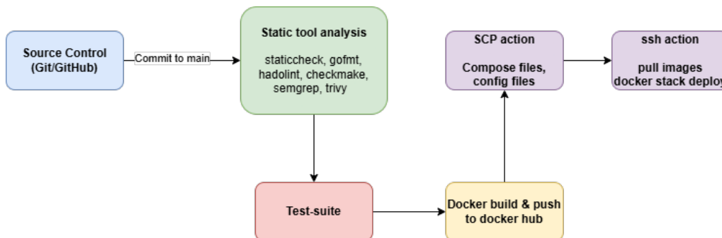
Figure 5: Overview of the CI/CD pipeline
