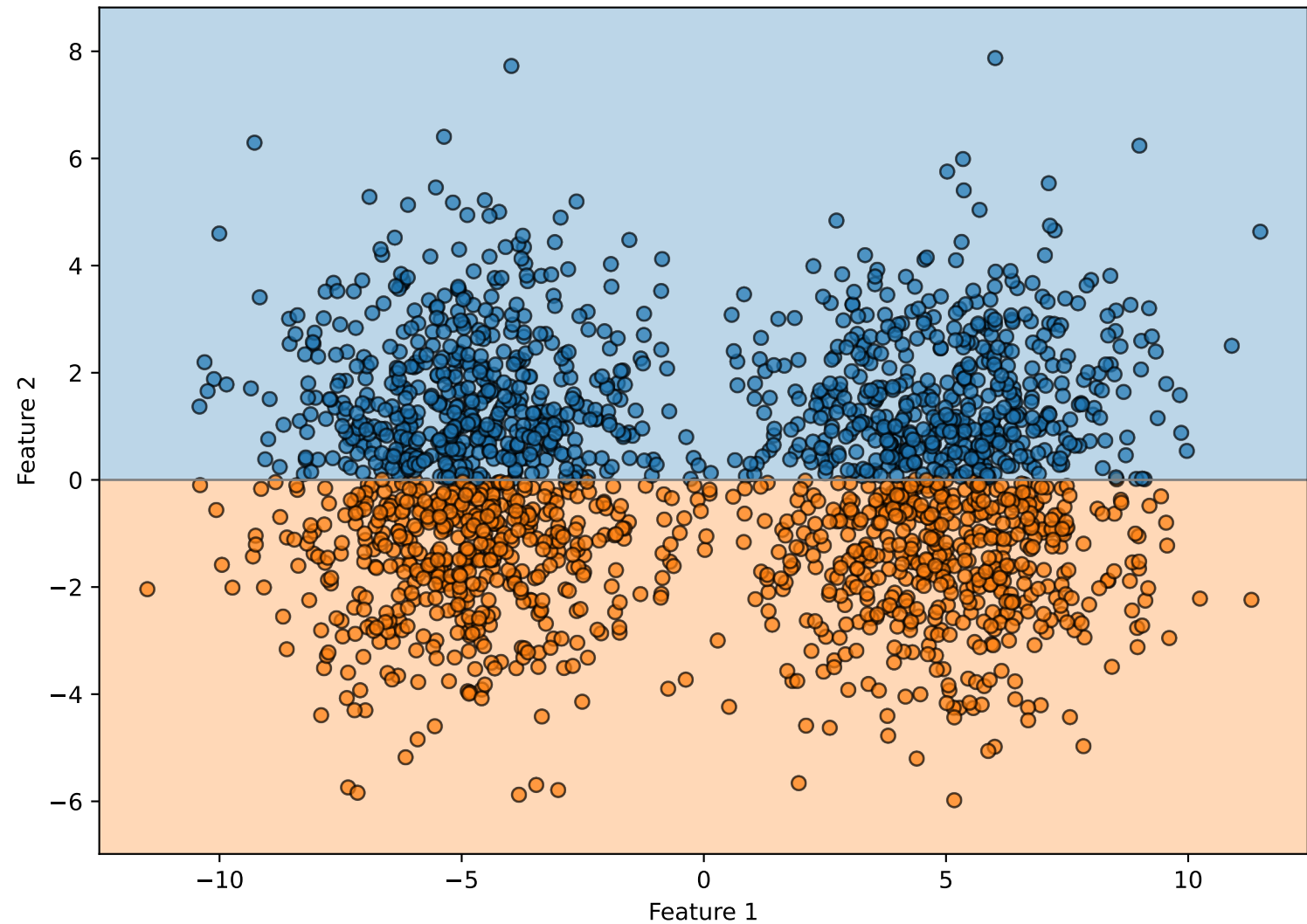
Decision Boundary
