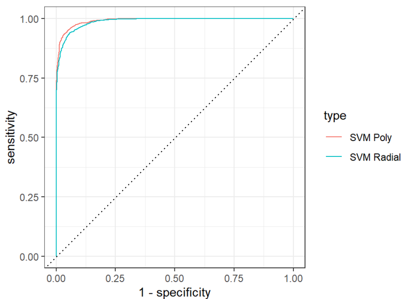
Figure 1: ROC Curves of SVM models.
