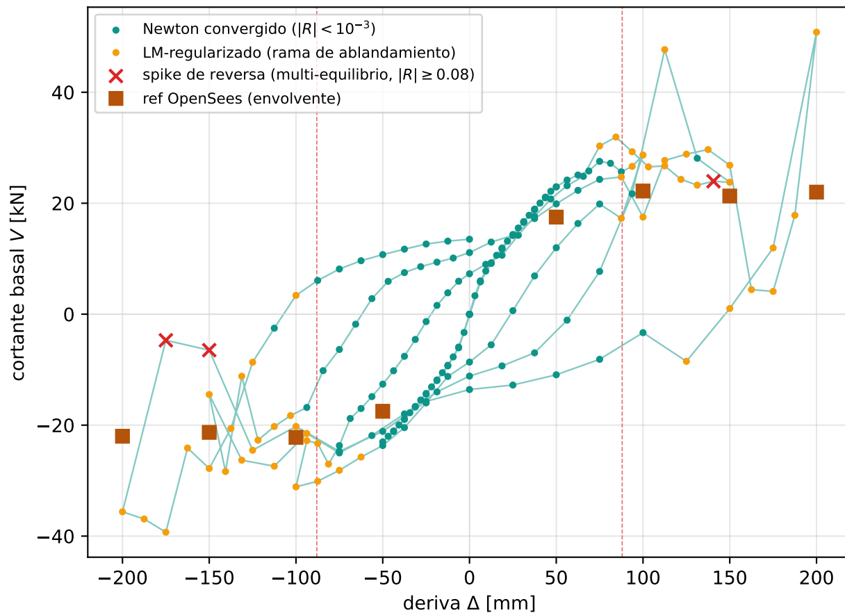
(a) Lazo ciclico 50/100/150/200 mm
