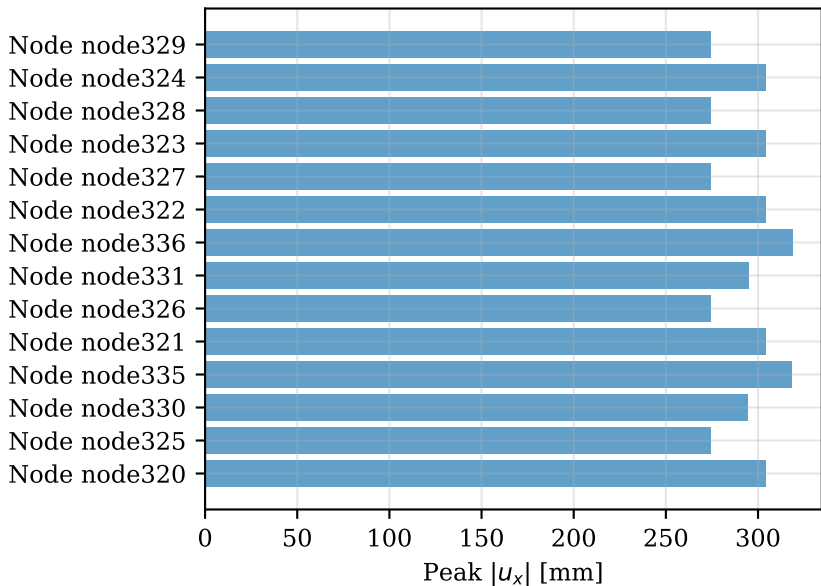
Peak lateral displacement envelope
