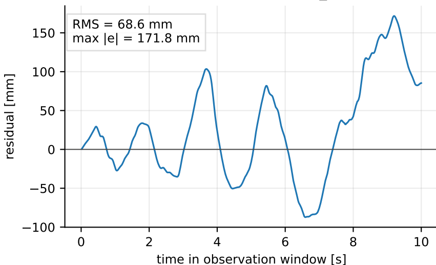
Residual OpenSees - fall_n, u_z
