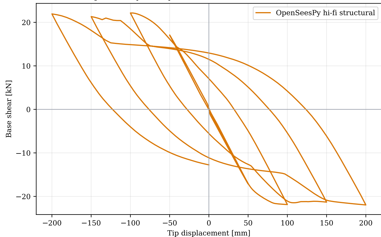
OpenSeesPy hi-fi cyclic RC-column reference to 200 mm
