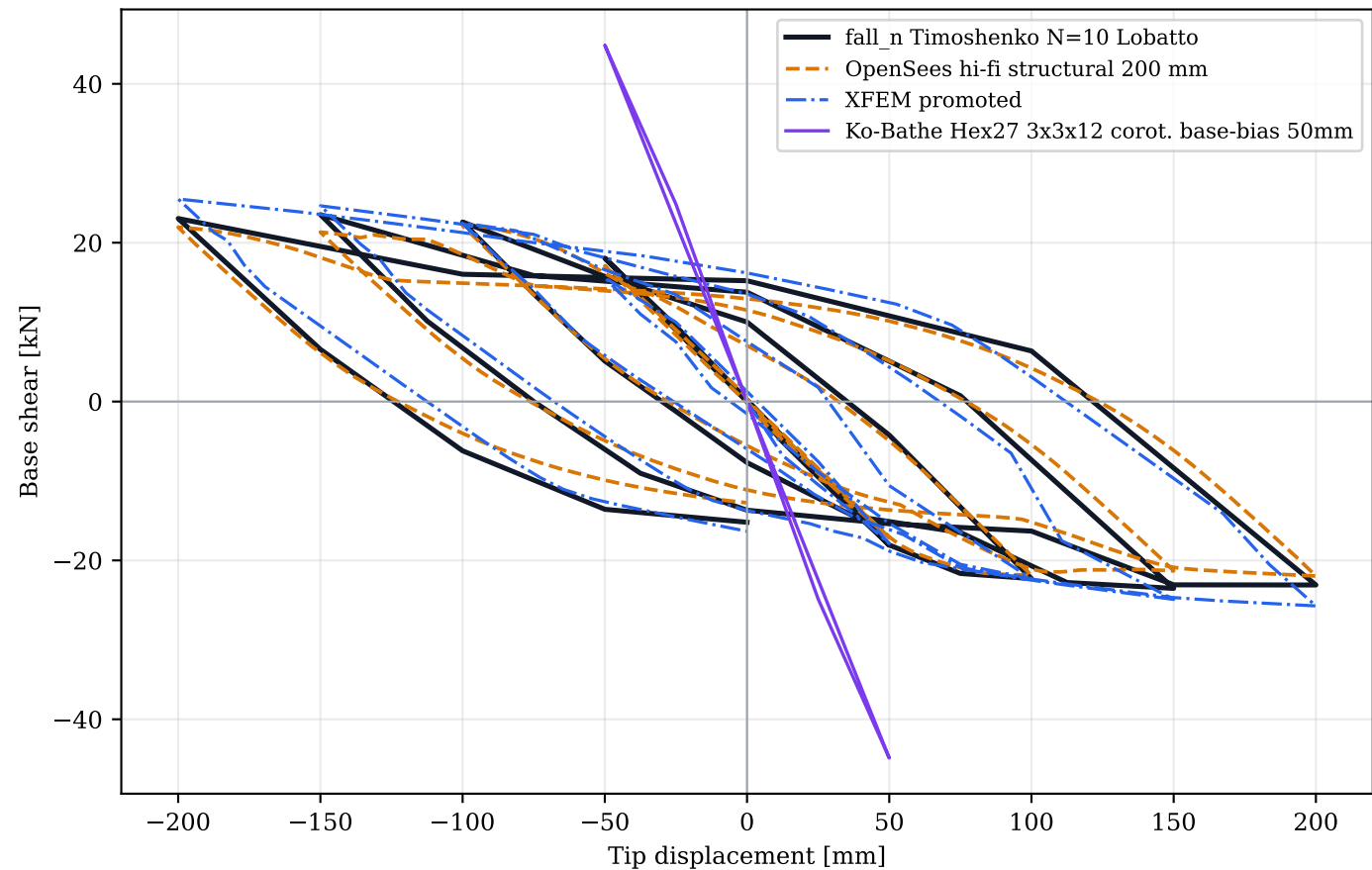
Cyclic RC-column hysteresis: structural, OpenSees hi-fi, and local models
