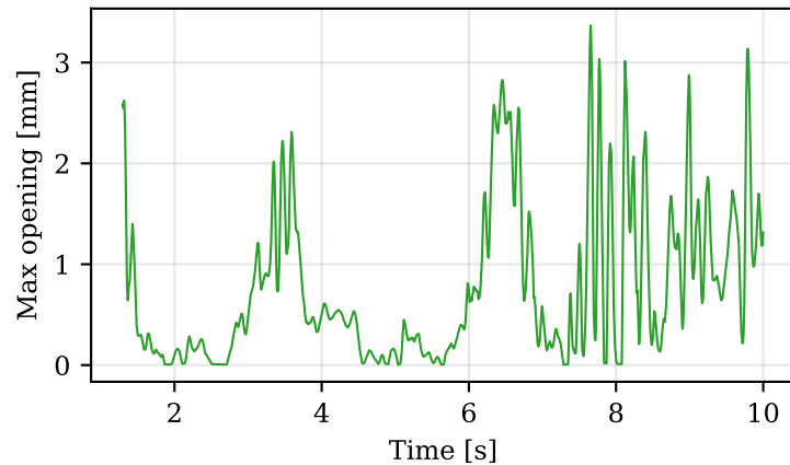
Max crack opening
