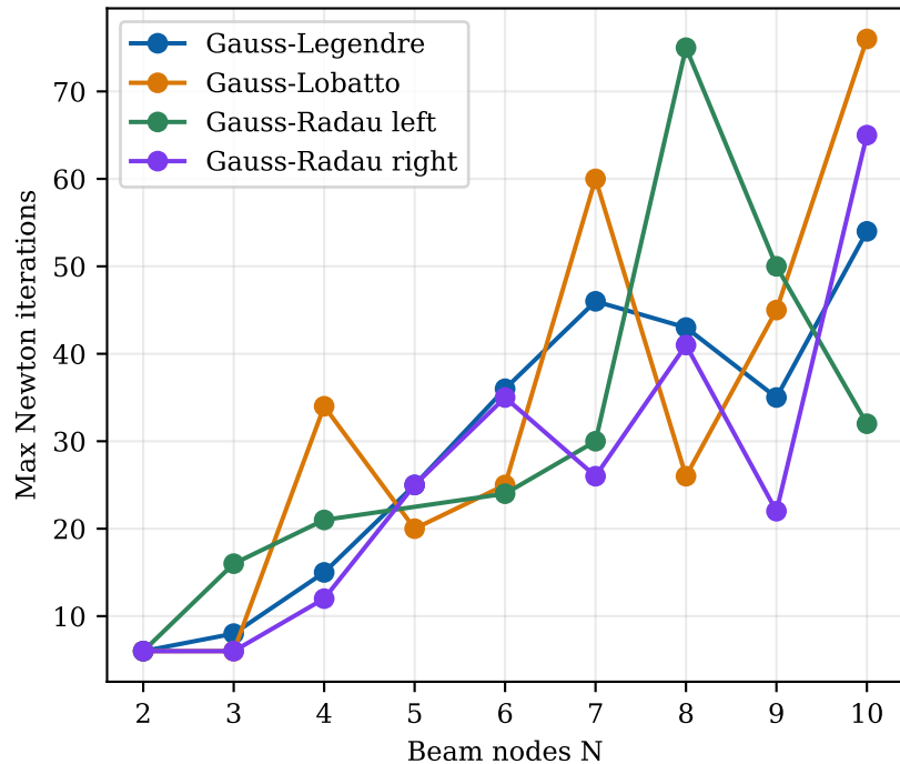
TimoshenkoBeamN matrix convergence
