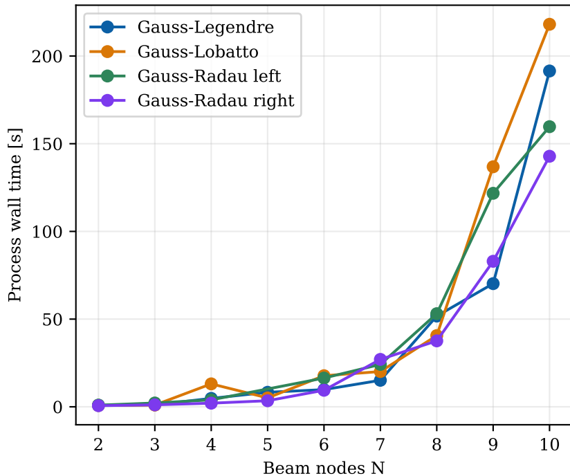
TimoshenkoBeamN matrix timing
