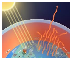
Greenhouse effect
