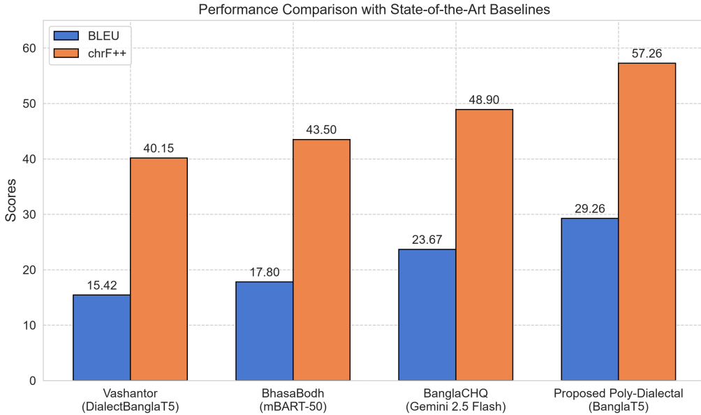
Figure 9: Visual comparison of BLEU and chrF++ scores across baseline systems and the proposed approach.
