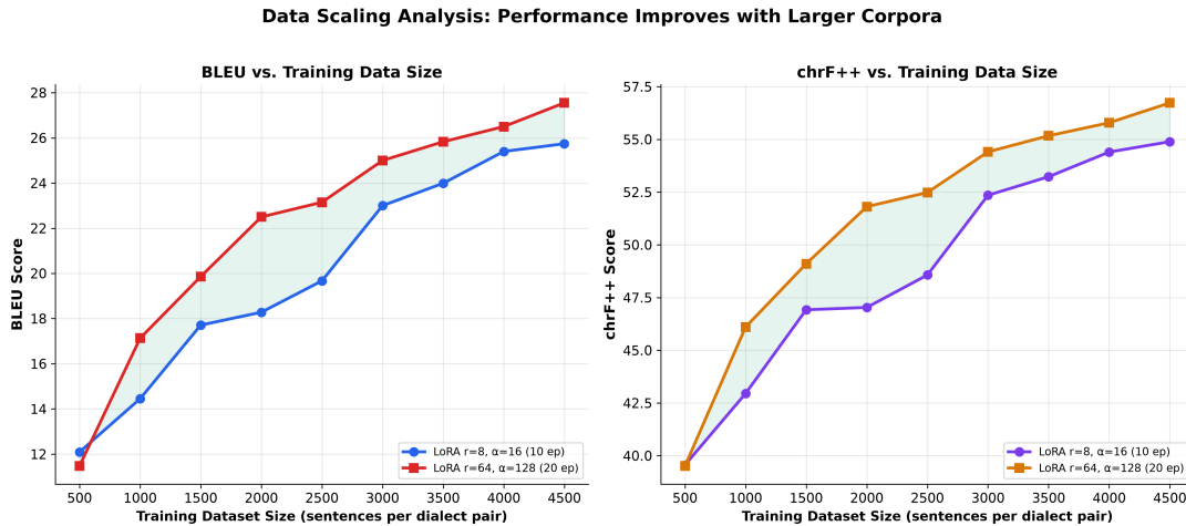
Figure 8: BLEU and chrF++ as a function of training data volume for two LoRA configurations. Consistent improvement is observed, with diminishing returns beyond approximately 3,000 samples.
