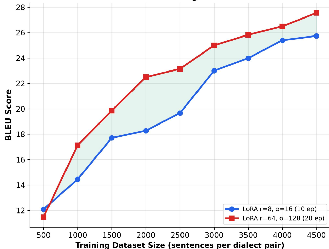
BLEU vs. Training Data Size
