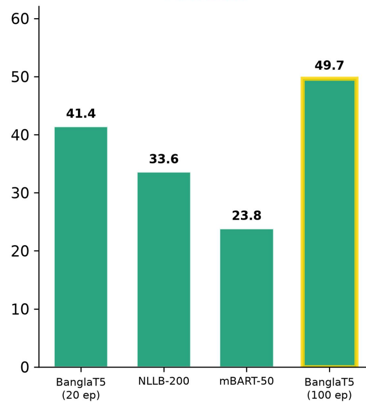
METEOR
