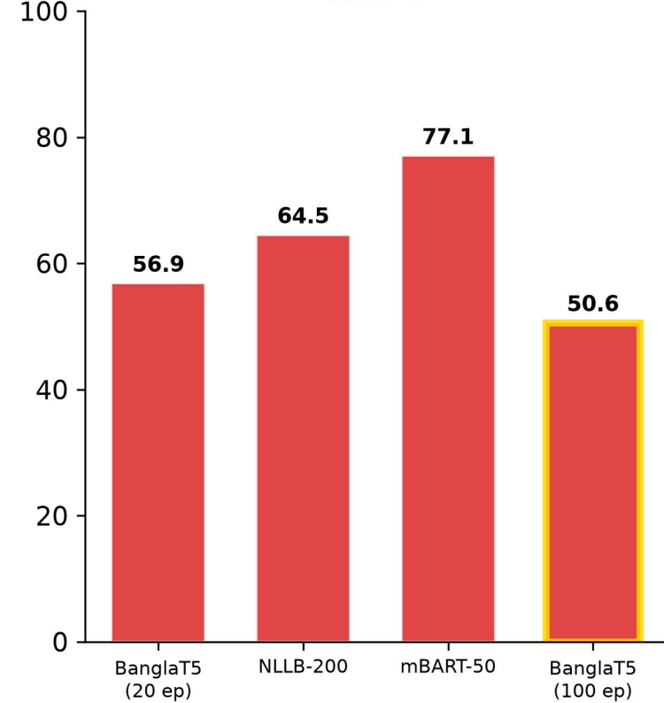
TER ↓
