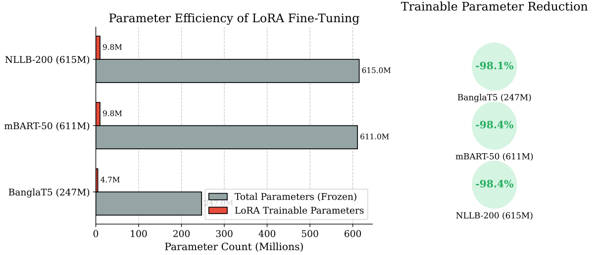
Figure 6: Parameter efficiency of LoRA fine-tuning across the three evaluated model architectures, demonstrating over 98% reduction in trainable parameters. Furthermore, we extend our methodology by introducing Weight-Decomposed Low-Rank Adaptation (DoRA) [18], which decomposes the pre-trained weights into magnitude and directional components for fine-tuning. This approach maintains the parameter efficiency of LoRA while achieving learning capacity closer to full fine-tuning. A visual comparison distinguishing LoRA’s structure from DoRA’s decomposed optimization is provided in Figure 6.
