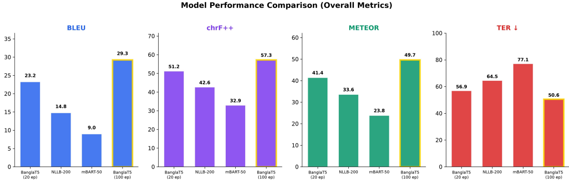
Figure 7: Comparative evaluation across experimental phases. BLEU [24], chrF++ [26], and METEOR [1] (higher is better) and TER [31] (lower is better) are shown for all three models at 20 epochs and BanglaT5 [2] at 100 epochs.
