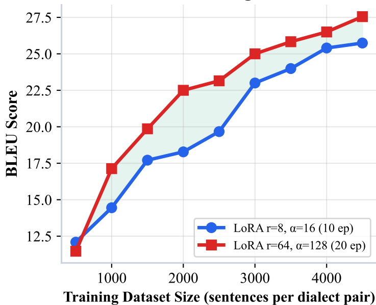
BLEU vs. Training Data Size
