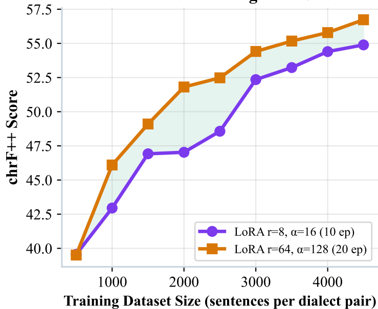
chrF++ vs. Training Data Size
