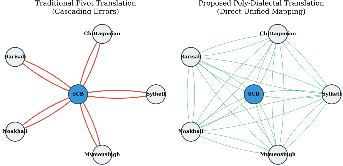
Figure 1: Structural comparison between the traditional pivot translation approach (routing through Standard Bangla) and the proposed direct poly-dialectal mapping topology.
