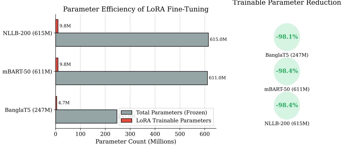
Figure 6: Parameter efficiency of LoRA fine-tuning across the three evaluated model architectures, demonstrating over 98% reduction in trainable parameters.
