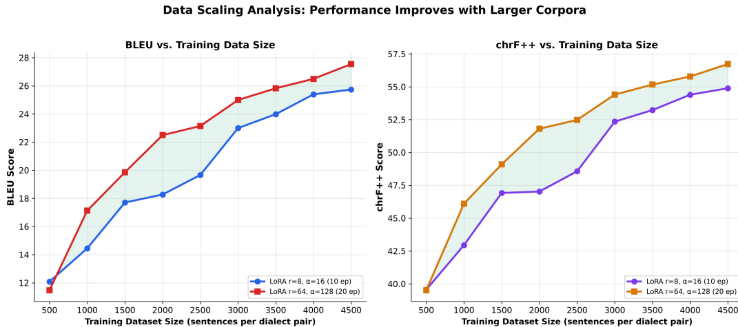
Figure 12: BLEU [23] and chrF++ [25] as a function of training data volume for two LoRA [10] configurations. Consistent improvement is observed, with diminishing returns beyond approximately 3,000 samples.
