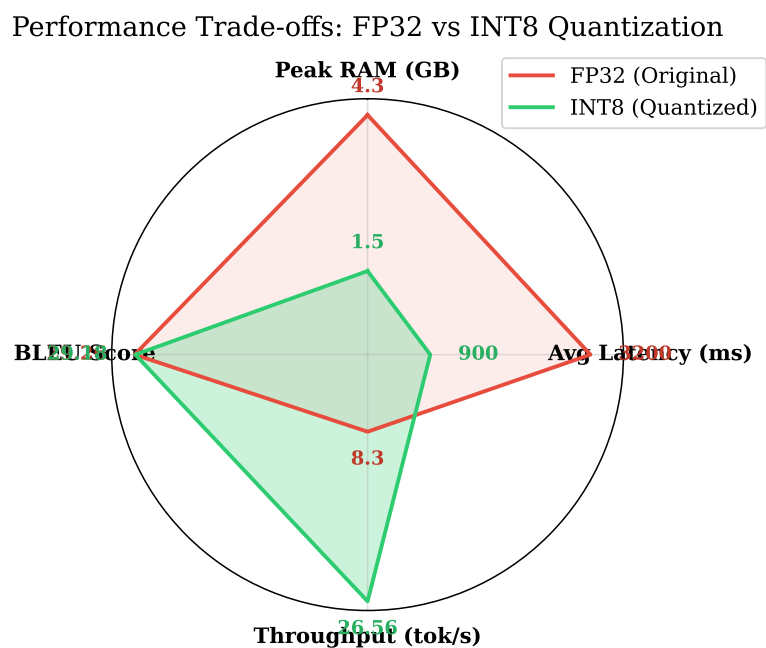
Figure 14: Multidimensional performance trade-off (Radar chart) demonstrating the advantages of INT8 quantization in reducing latency and memory footprint while preserving translation quality.
