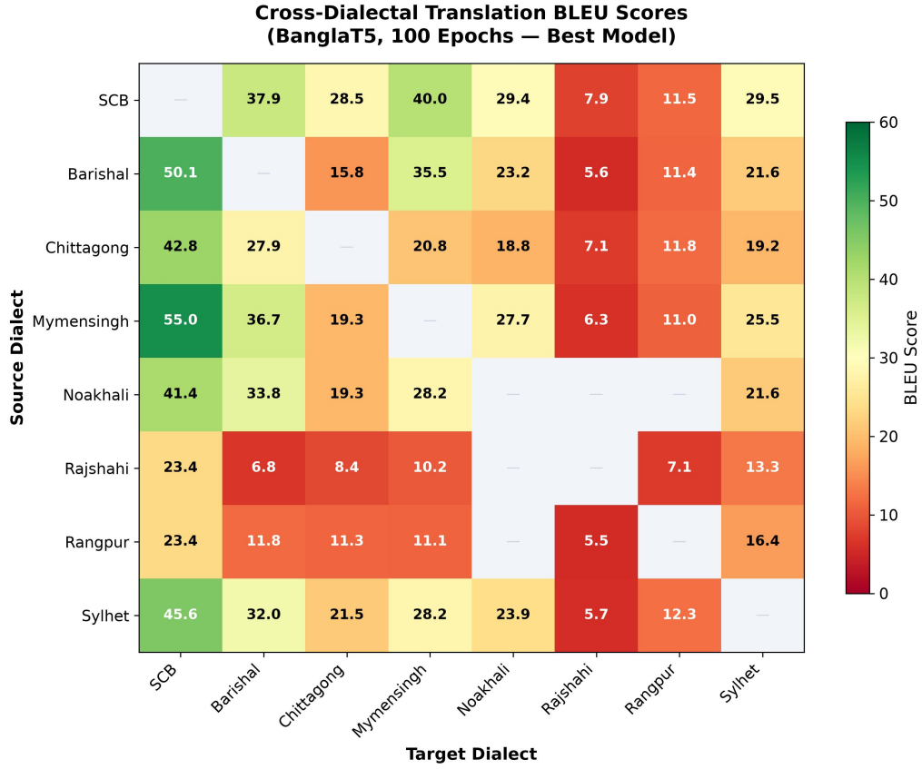
Figure 8: Cross-dialectal BLEU [23] score heatmap (BanglaT5 [2], 100 epochs). Darker shading indicates higher translation quality. Low-resource dialects (Rajshahi, Rangpur) exhibit uniformly lower scores, while morphologically proximate pairs (Mymensingh↔SCB) achieve the highest scores.
