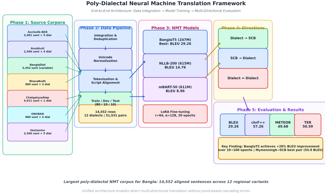
Figure 2: End-to-end architectural workflow of the Poly-Dialectal Neural Machine Translation Framework, depicting five phases: source corpora integration from seven existing datasets, the data processing pipeline, NMT model fine-tuning with LoRA, multi-directional translation paradigm, and evaluation with four standard MT metrics.
