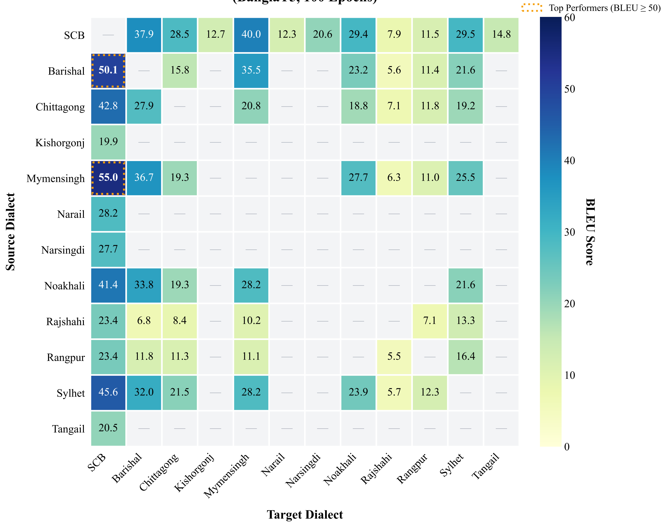
Cross-Dialectal Translation BLEU Scores (BanglaT5, 100 Epochs)
