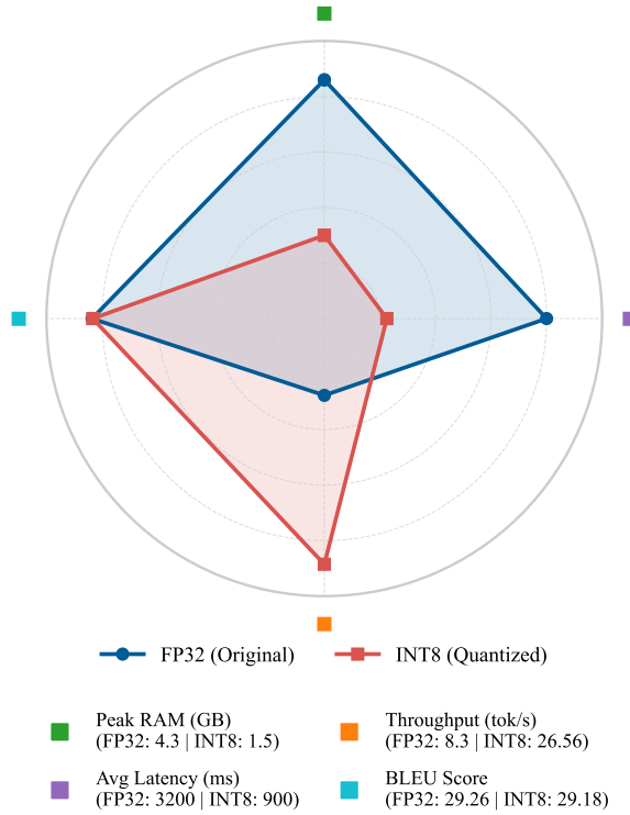
Performance Trade-offs: FP32 vs INT8
