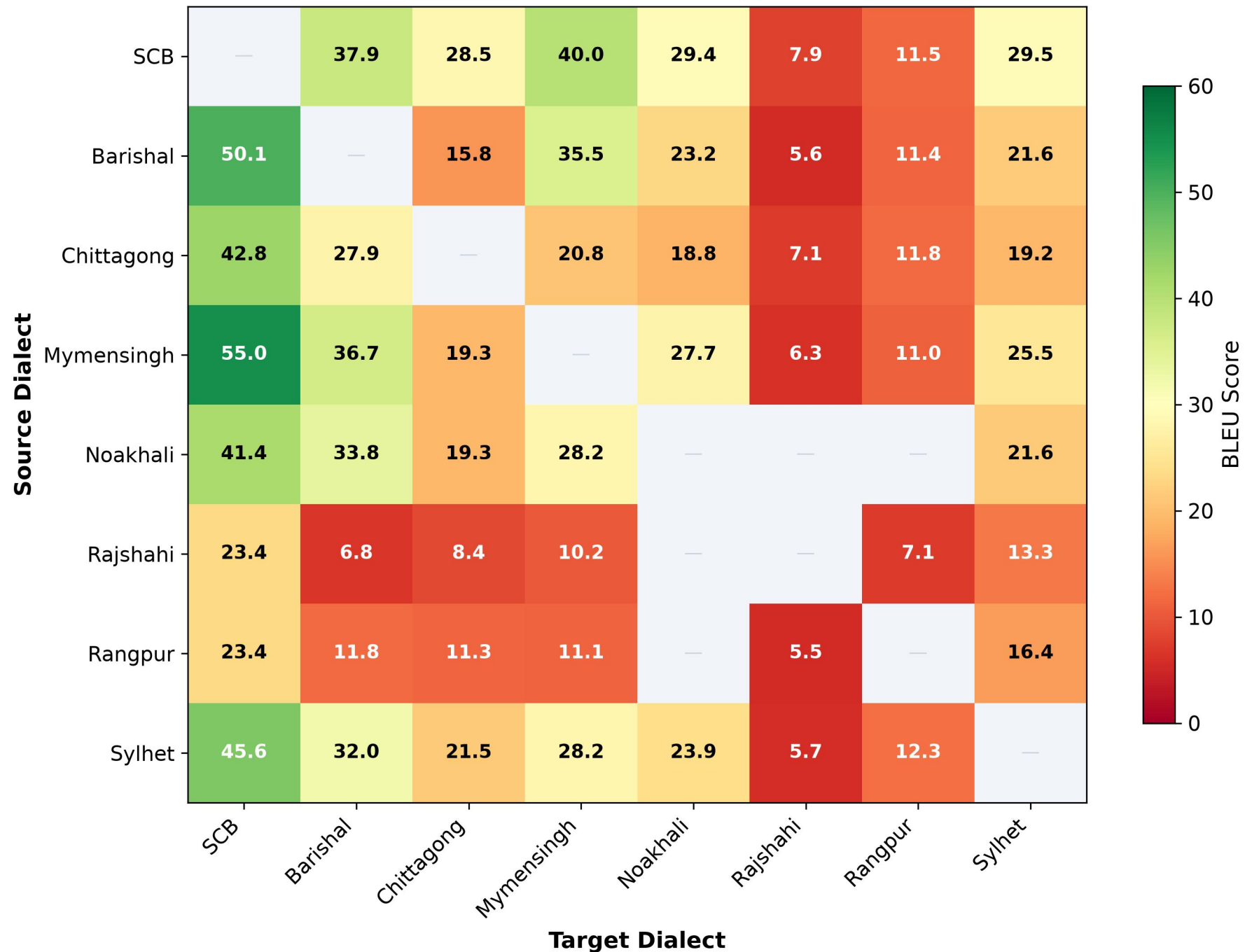
Cross-Dialectal Translation BLEU Scores (BanglaT5, 100 Epochs — Best Model)
