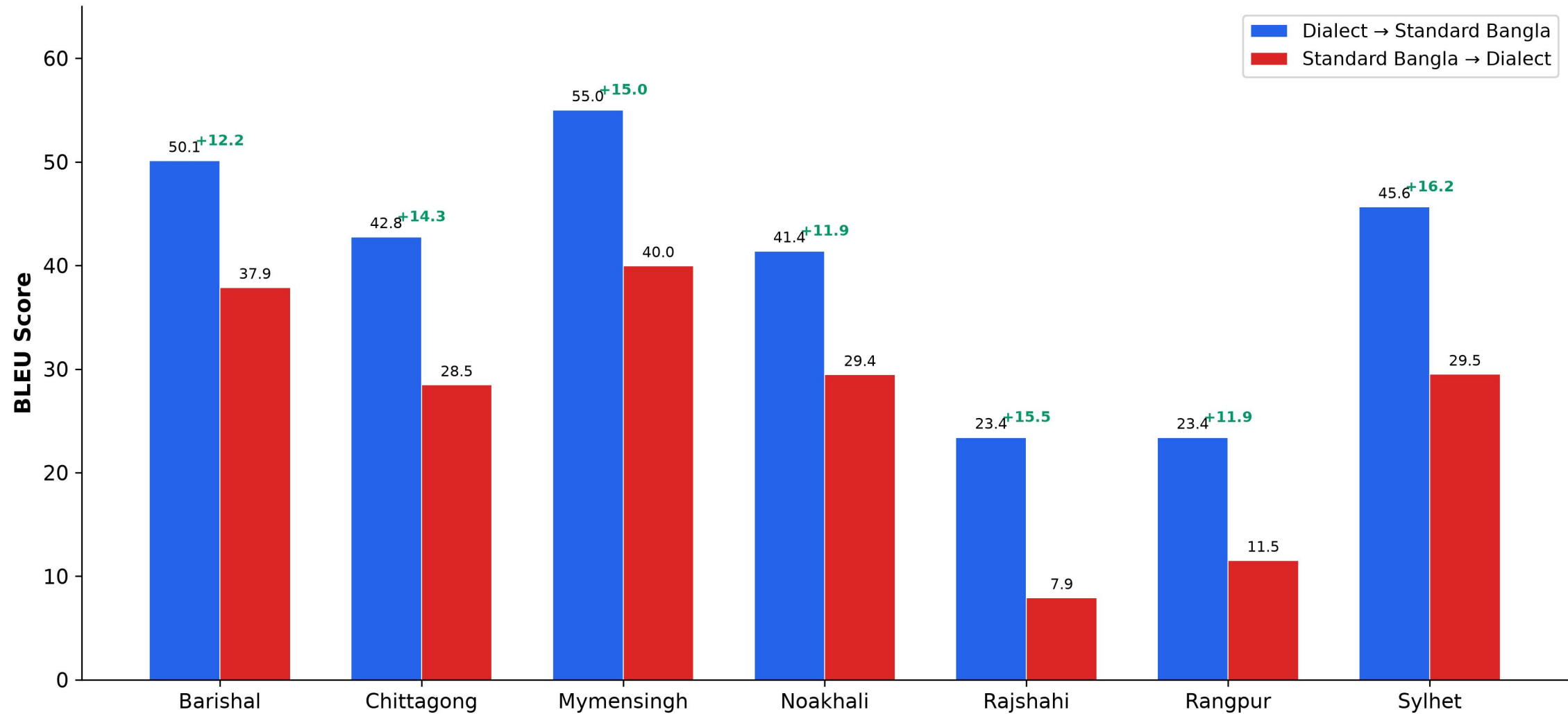
Translation Directionality Asymmetry (BanglaT5, 100 Epochs)
