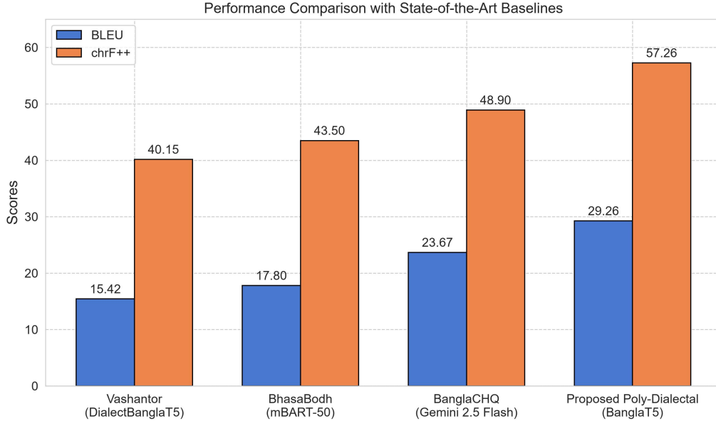
Figure 14: Visual comparison of BLEU [24] and chrF++ [26] scores across baseline systems and the proposed approach.
