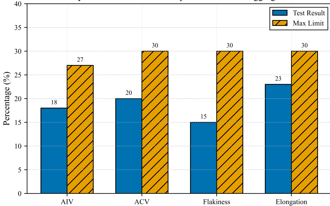
Physical and Mechanical Properties of Coarse Aggregates
