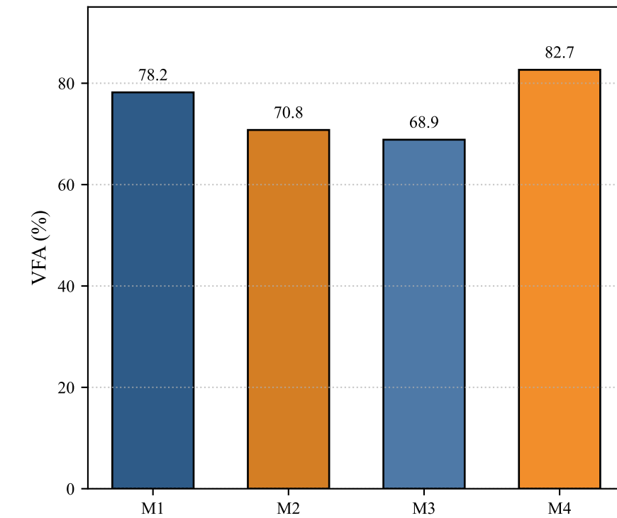
Voids Filled with Asphalt (VFA)
