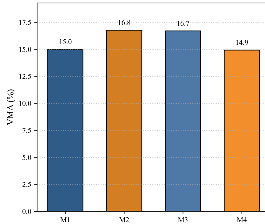
Voids in Mineral Aggregate (VMA)
