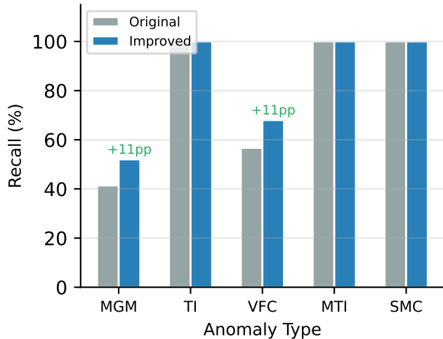
(b) Per-type Improvement
