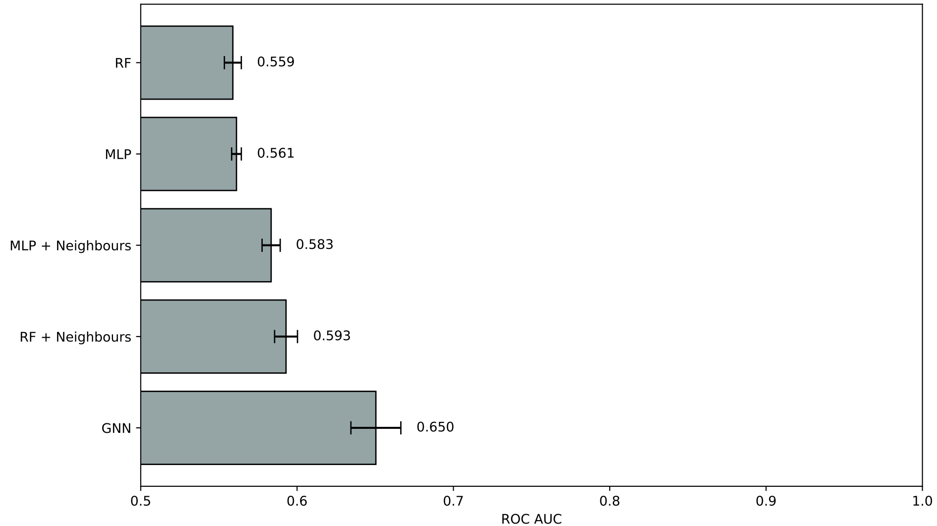
GNN vs Baseline Classifiers
