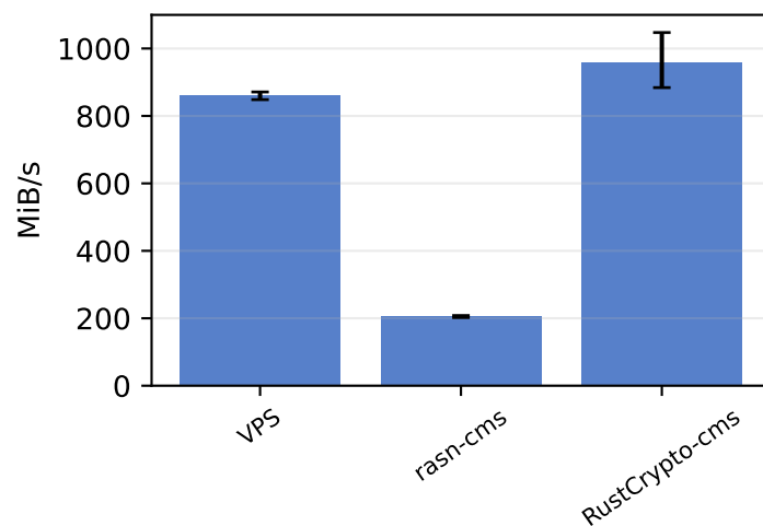
CMS RFC 4134 — serialize
