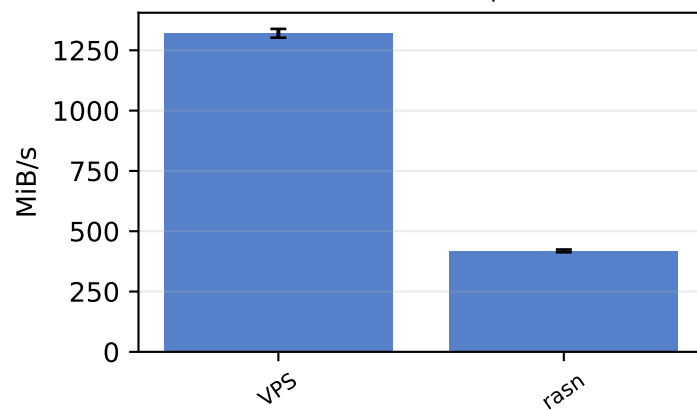
ASN.1 BER normalized output — serialize
