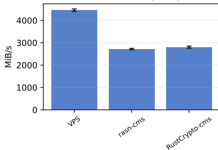
CMS combined real corpus — parse
