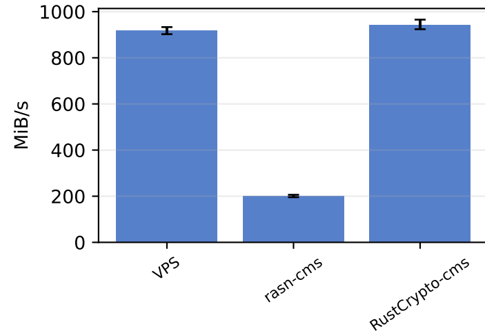
CMS NIST PKITS — serialize
