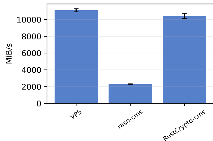
CMS EC DSS CADES — serialize
