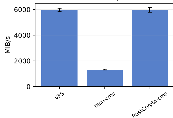
CMS combined real corpus — serialize
