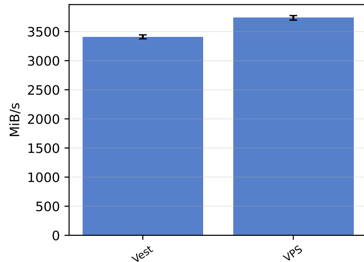
tls — serialize
