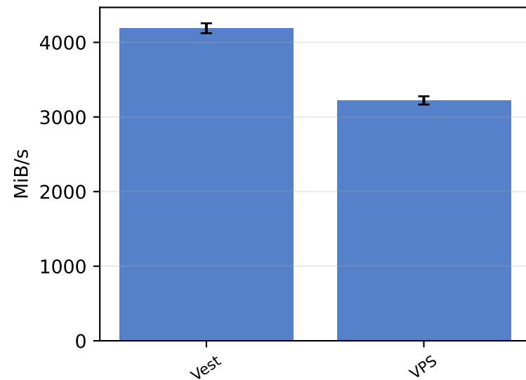
tls — serialize
