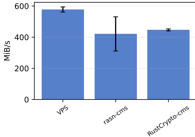
CMS NIST PKITS — parse
