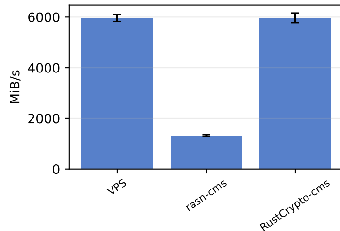
CMS combined real corpus — serialize
