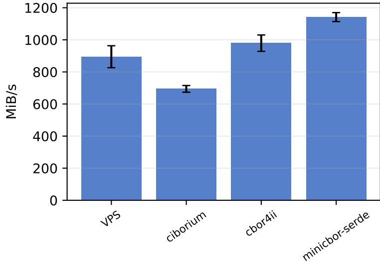
CBOR — serialize
