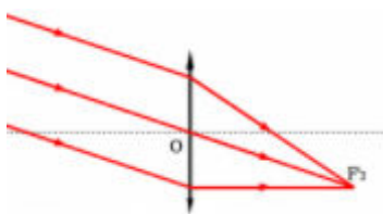
FIGURE 1 – Foyer secondaire lentille convergente
