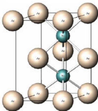
FIGURE 12 – Coordination anions-cations
