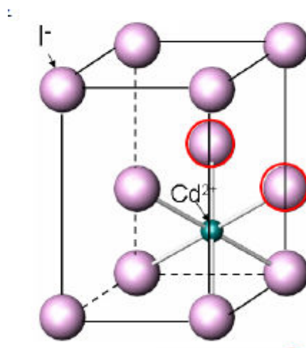
FIGURE 14 – Coordinance anions-cations
