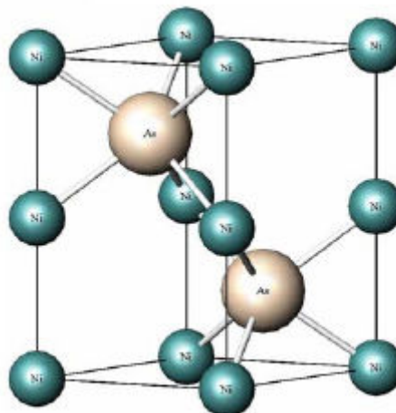
FIGURE 13 – Coordination cations-anions
