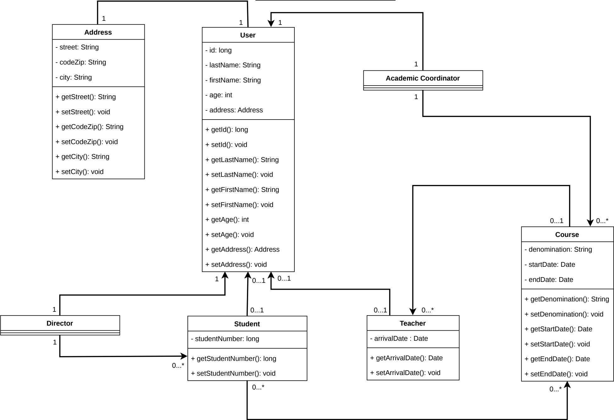
Class diagram School Management
