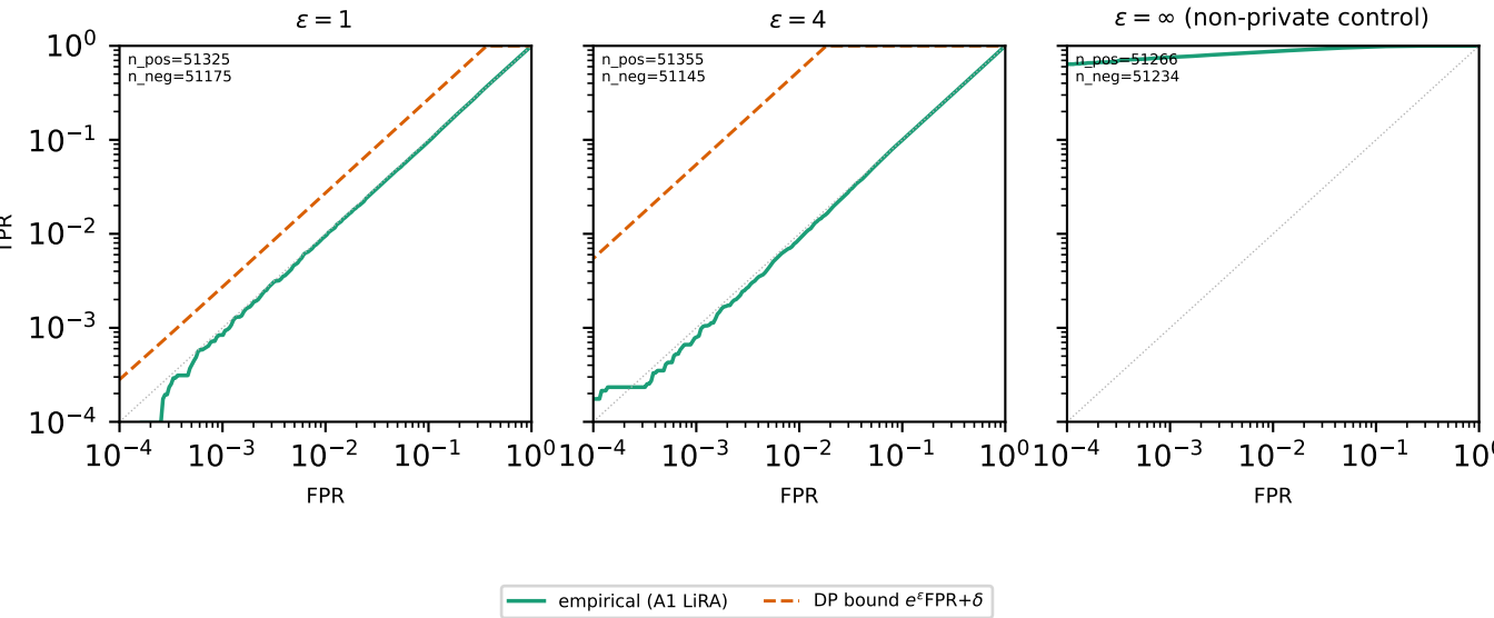
FIG10 — M9 audit: empirical LiRA vs. the analytic DP bound (Theorem 11)
