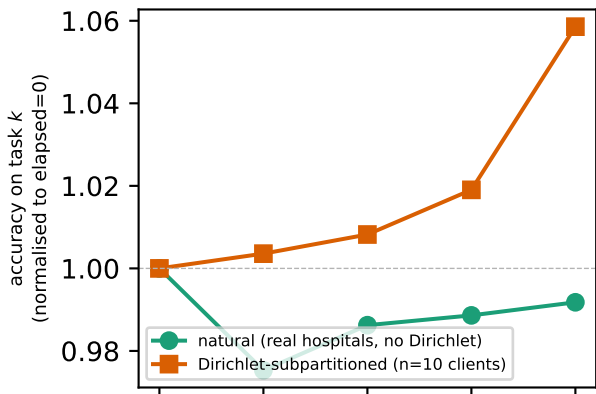
FIG18 (PILOT) — Camelyon17: natural vs. Dirichlet client partition, M0
