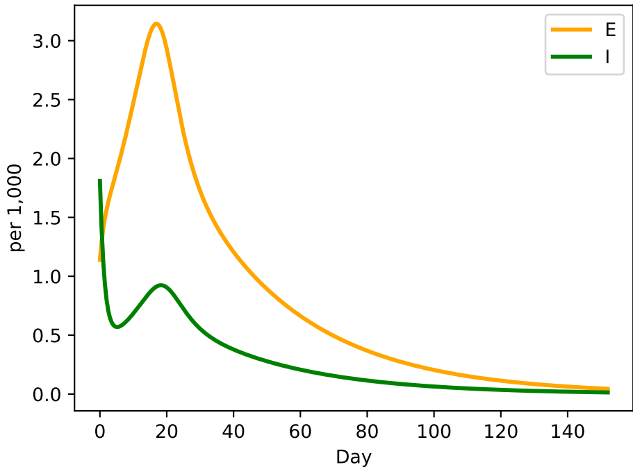
Exposed & Infectious
