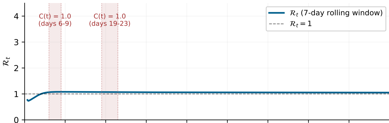
S1-A Time-varying \mathcal{R}_t — conflict peaks highlighted
