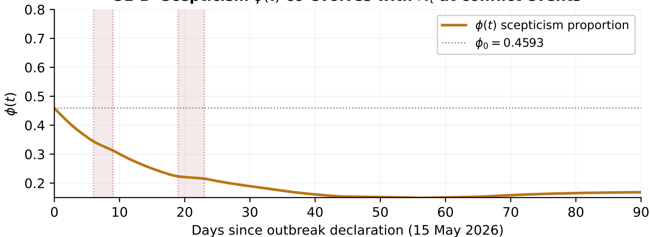
S1-B Scepticism \phi(t) co-evolves with \mathcal{R}_t at conflict events
