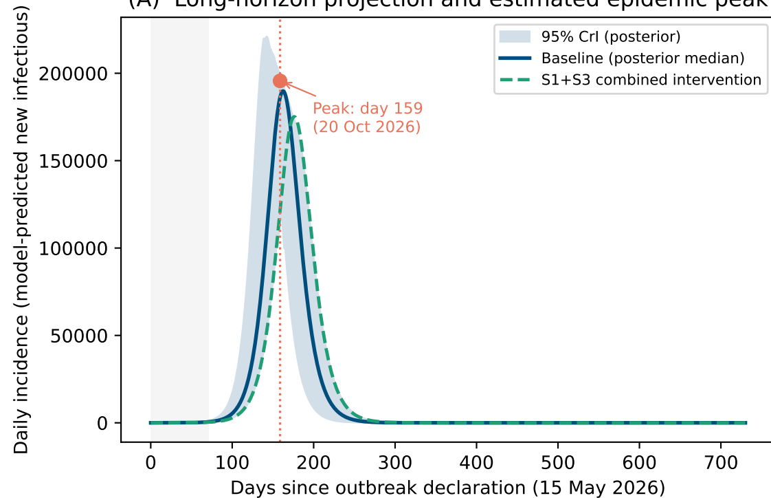
(A) Long-horizon projection and estimated epidemic peak
