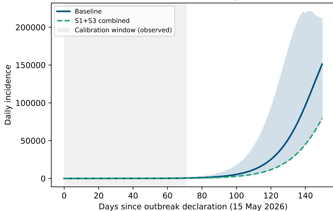
(B) Near-term window (days 0-150)
