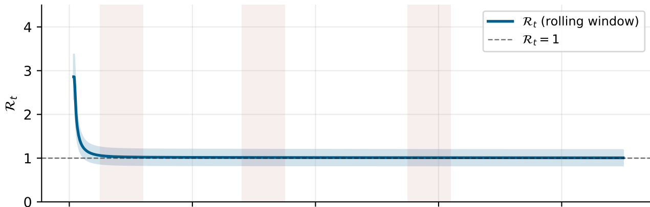
S1-A Time-varying \mathcal{R}_t — conflict pulses highlighted
